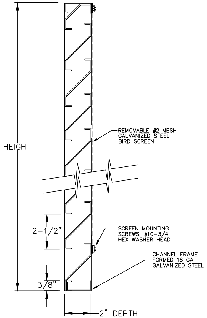
VERTICAL SECTION
