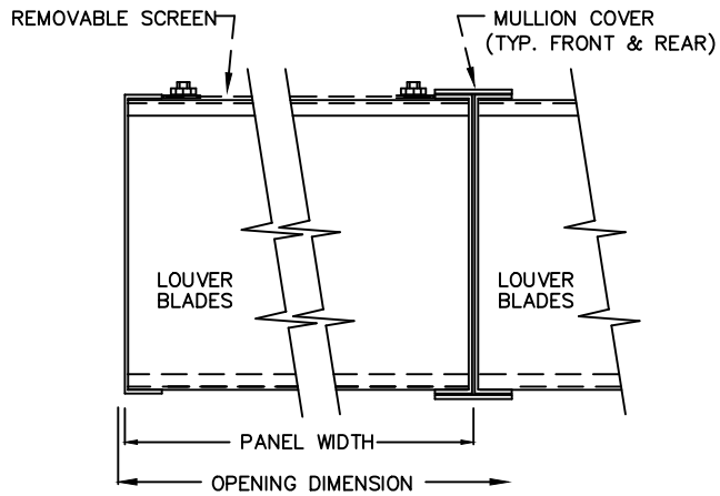
HORIZONTAL SECTION
