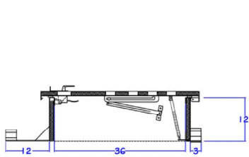
STANDING SEAM BASE OPTION
