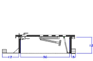
SEAM CLIP BASE OPTION
