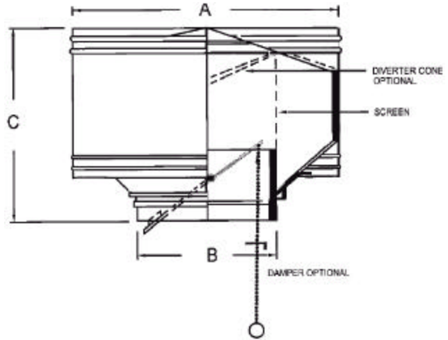
DIMENSION - GAUGES
