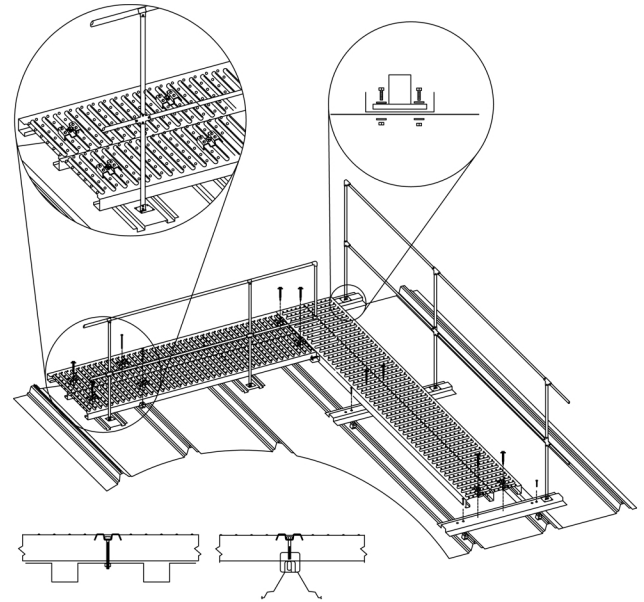
RW24 STANDING SEAM
