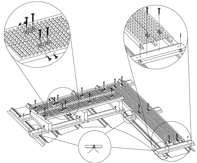
RW24 PITCHED CORRECTED STANDING SEAM
