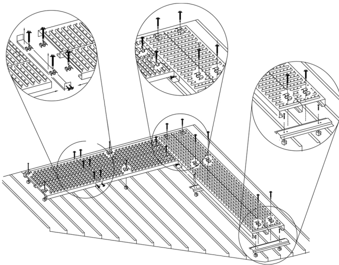
RW24 BATTEN STANDING SEAM
