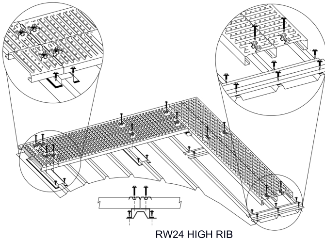
RW24 HIGH RIB
